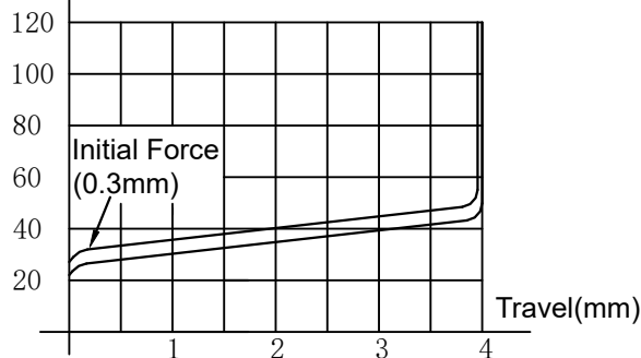
Force-Travel-Diagram
