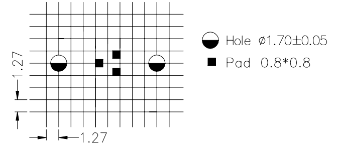
Layout of PCB
