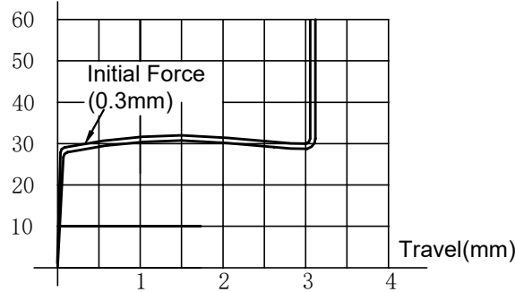
Force-Travel-Diagram
