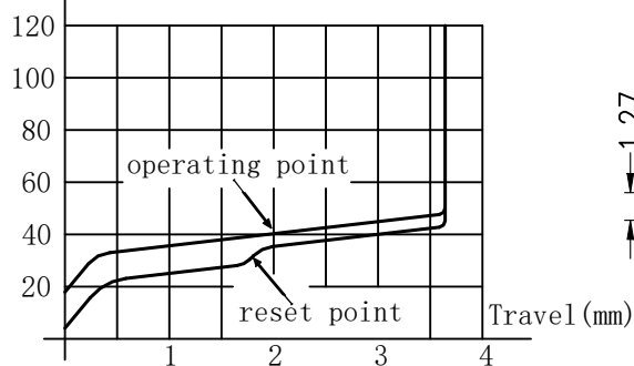
Force-Travel-Diagram
